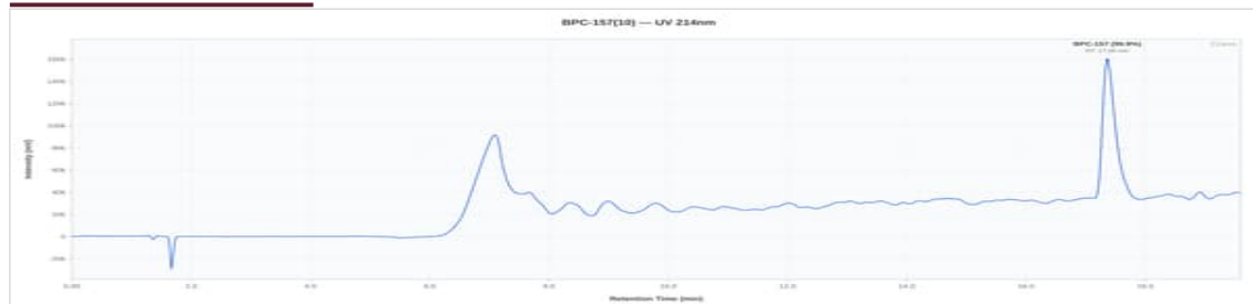
BPC-157 10mg - ELU202606-BPC10: UV Chromatogram
