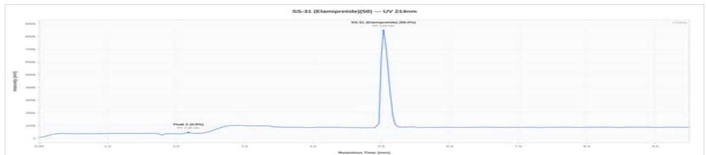
SS-31 50mg - 202607-SS50: UV Chromatogram
