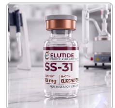
SS-31 50mg - 202607-SS50
